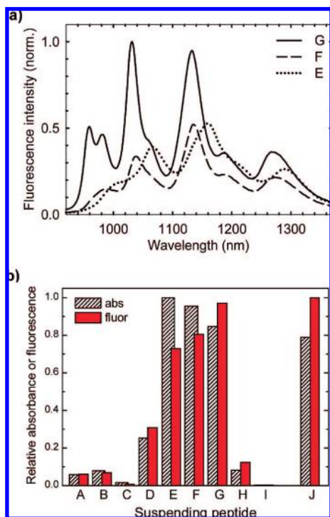
Figure 2. (a) Fluorescence emission spectra from bulk SWCNT samples suspended in peptide coatings E, F, and G. The spectra have been normalized to the most intense peak in peptide G. (b) Average spectrally integrated fluorescence emission and absorbance for bulk SWCNT samples suspended in the family of peptide coatings A–I, and in peptide J (normalized to the maximum values).
