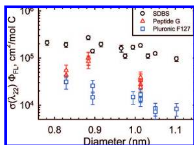
Figure 6. Measured fluorescence action cross sections of selected SWCNT structures suspended in aqueous SBDS (○), peptide K_2(\text{QL})_5K_2 (G) (△), and Pluronic F127 (□). Data for SWCNTs in SBDS are taken from ref 9.
